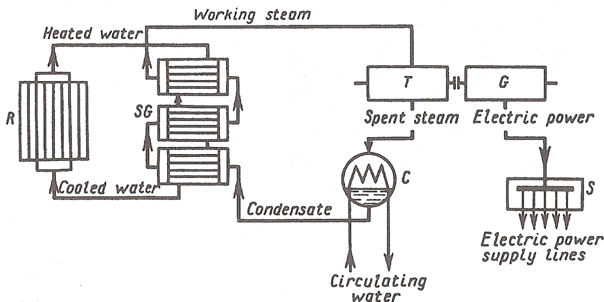
Simplified production process diagram of nuclear power plant:
